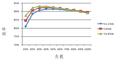
RSD-300B-48
