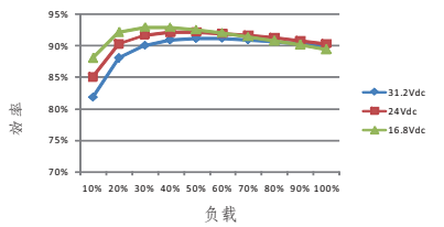
RSD-300C-5
