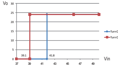
RSD-300F-24
