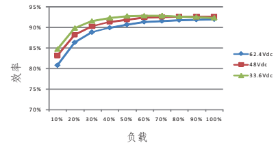
RSD-300D-24
